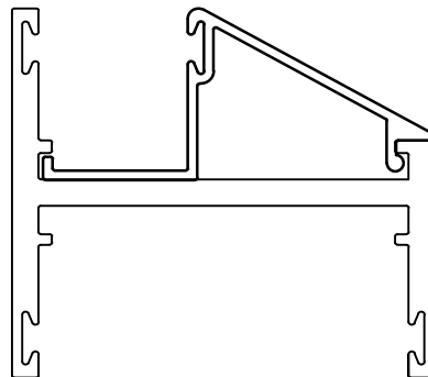
1/2" Bevel Stop
