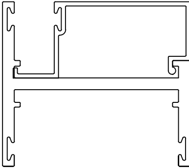
1/4" Square Stop
